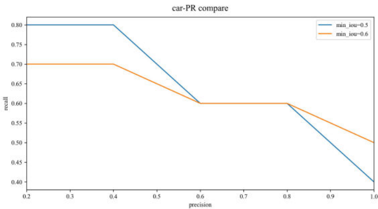
图 5-16 car-PR compare
